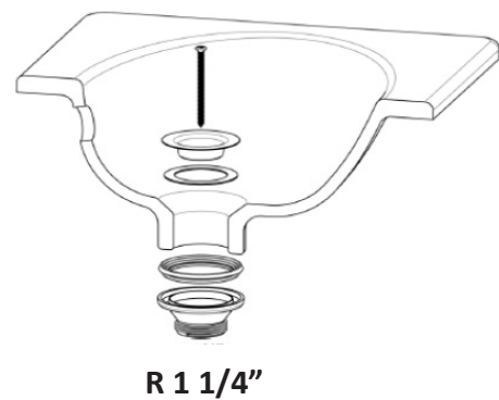
Waste valve assembly
